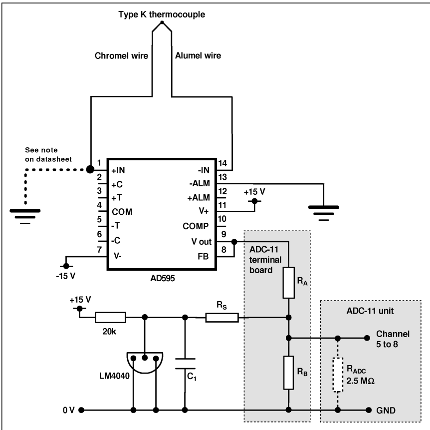
Temperature sensor circuit with thermocouple and AD595
